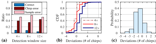
Figure 6: (a,b) Deviations of detected frame timing with different detection windows (DW); (c) Histogram of timing deviations (DW=4x).
