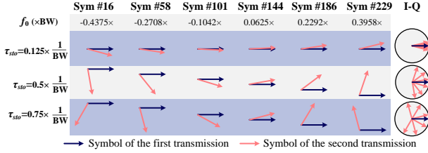
Figure 10: Illustration of signal combination for LoRa symbols in various STO differences ( \Delta\tau_{sto} ).
