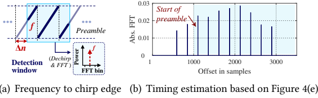
Figure 5: Coarse estimation of frame timing.
