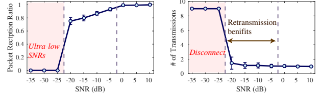
(a) Packet Reception Ratio (PRR) (b) Packet transmission times Figure 2: Performance of LoRaWAN retransmission in various SNRs (SF12, BW 125 kHz): MAC layer retransmission cannot benefit weak links ( e.g. , SNR < -20 dB).
