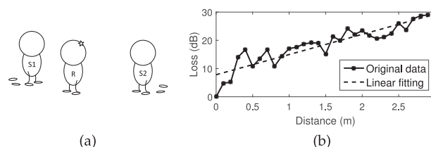
Fig. 14. For receiver R, the far sender’s signals are “overwhelmed” by near sender’s signals. The attenuation rate of acoustic signals is as high as 6.6 dB/m.
