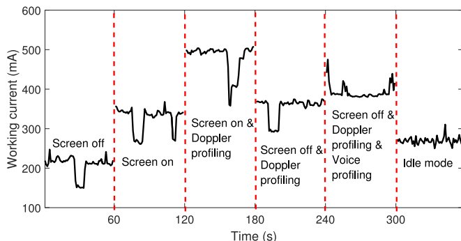
Fig. 21. Power profile of DopEnc.
