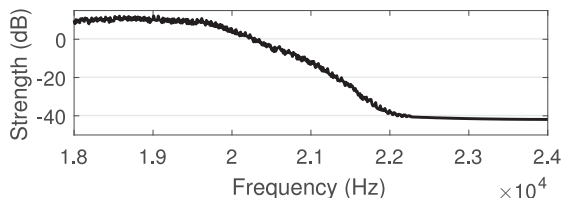
(a) Speaker of LG Nexus 5 to microphone of Samsung Galaxy Nexus i9250
