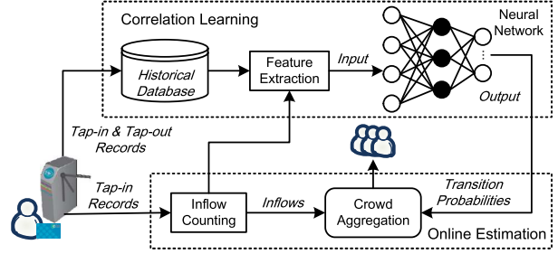
Fig. 6. Architecture of CrowdAtlas.
