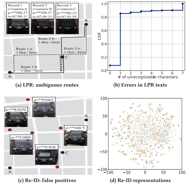
Figure 5: Impact of identity uncertainties on vehicle trajectory reconstruction
