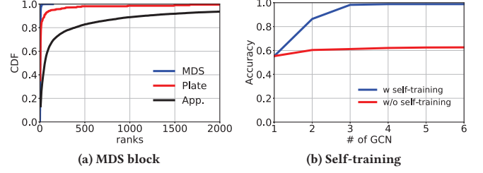
Figure 15: Performance of VeTrac components
